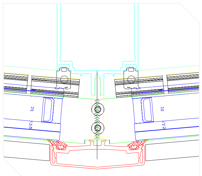
Curtain Wall Cross-Section
